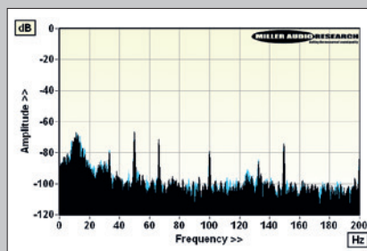
Fig.2 Unweighted rumble from DC- 200\text{Hz} (with clamp, blue; without clamp, black), all ref. 1\text{kHz} at 5\text{cm/s} .
