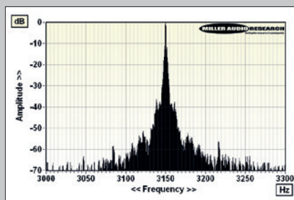
Fig.1 Wow and flutter re. 3150\text{Hz} tone at 5\text{cm/s} (plotted \pm 150\text{Hz} , 5\text{Hz} per minor division).
