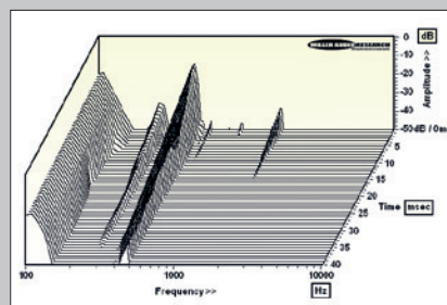
Fig.3 Cumulative spectral decay spectrum illustrating the tonearm's various bearing, pillar, and "tube" vibration modes 100\text{Hz--}10\text{kHz} over 40\text{ms} .
